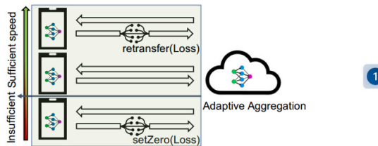
Fig. 15. The illustration of ThrowRightAway (TRA) scheme [155].
