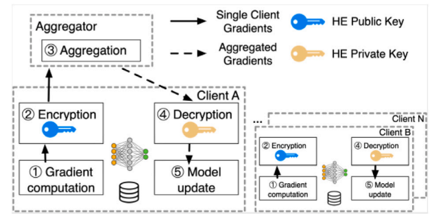
Fig. 12. The illustration of BatchCrypt [85].
