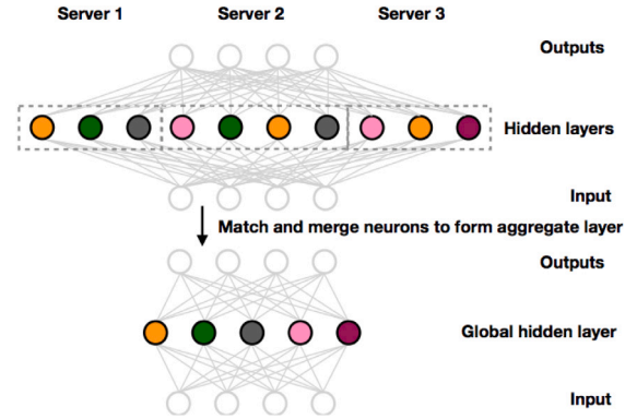
Fig. 4. The illustration of PFNM [99].
